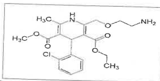
FIG. 1: CHEMICAL STRUCTURE OF AMLODIPINE BESYLATE
